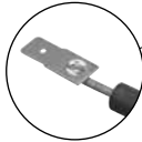
.250" male terminal push-in connection
