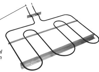
.250" male terminal push-in connection
