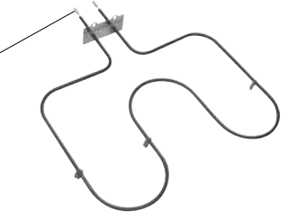
.250" male terminal push-in connection
