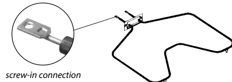
screw-in connection
